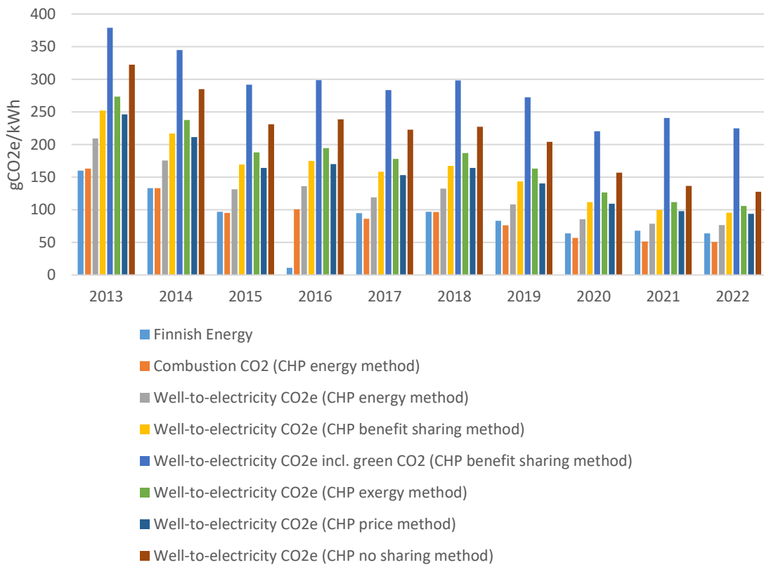
Electricity generation in Finland 2013–2022, gCO 2 e/kWh
