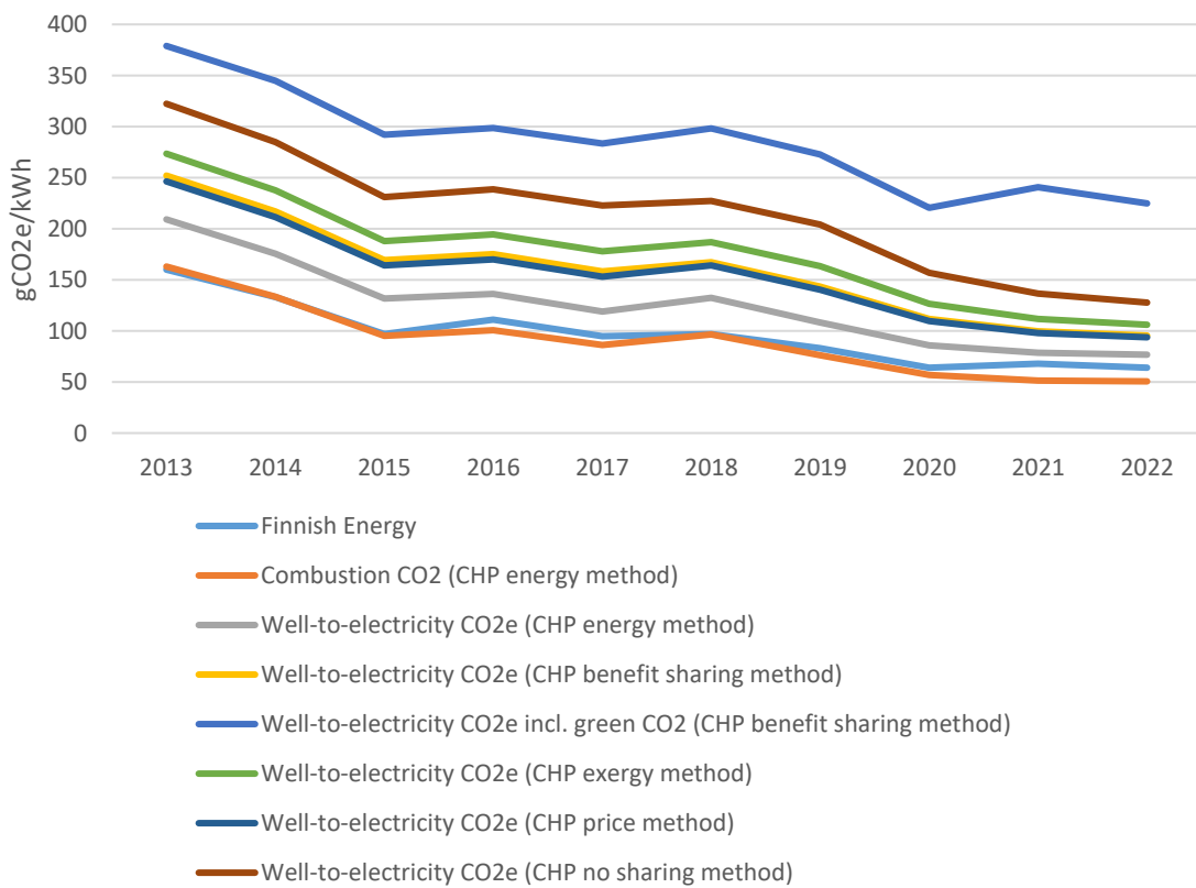
Electricity generation in Finland 2013–2022, gCO 2 e/kWh
