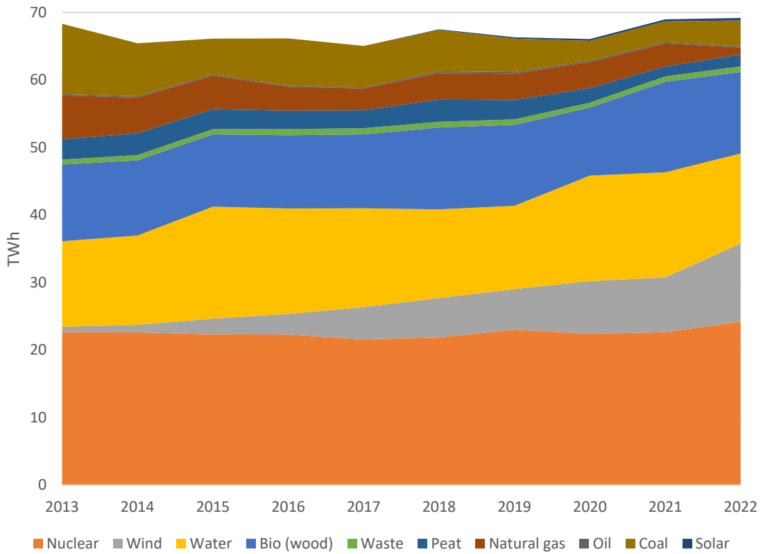
Electricity generation in Finland 2013–2022, TWh
